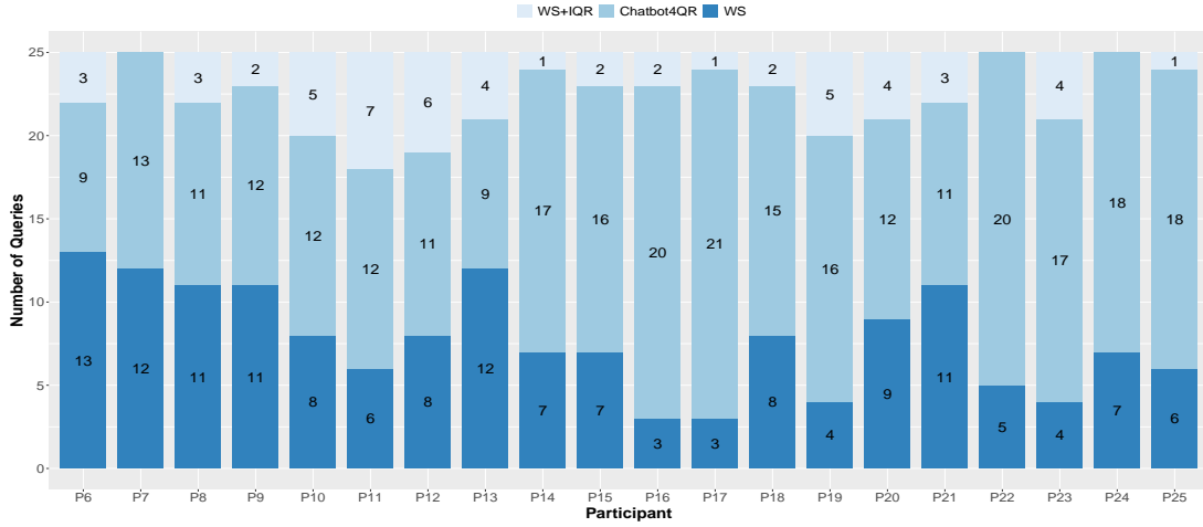
Fig. 9. The numbers of queries that achieve the best results using WS, WS+IQR, and Chatbot4QR by 20 participants.
